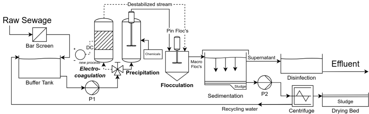
Figure 1: Hypothetical wastewater treatment process including EC, precipitation, and flocculation.
